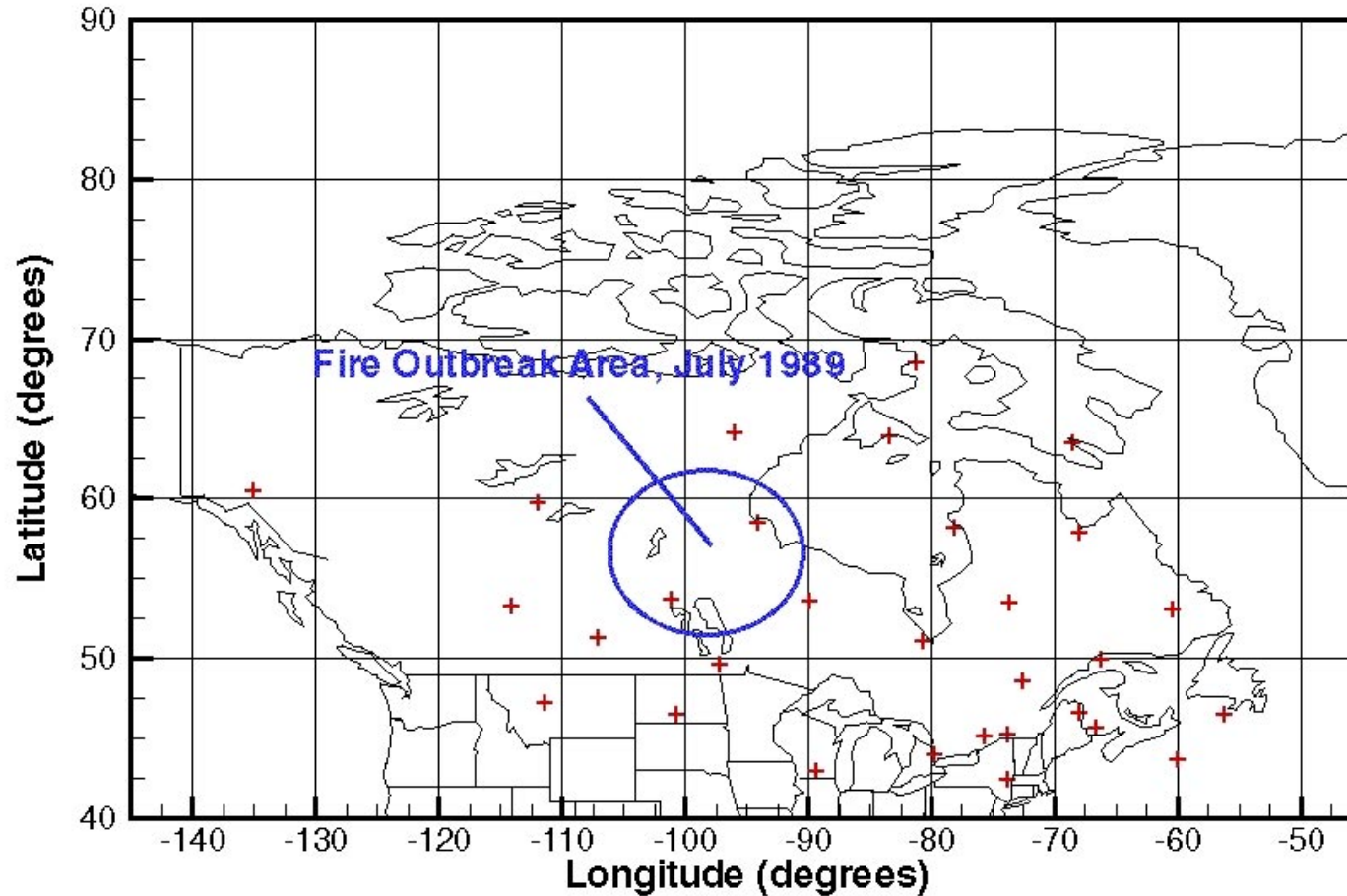
Figure 1: A map of Canada and Northern United States showing the main fire area outlined in blue for the July 1989 Boreal forest fire outbreak in Manitoba, Canada. The red crosses denote the locations of surface radiometers used in the case study.
