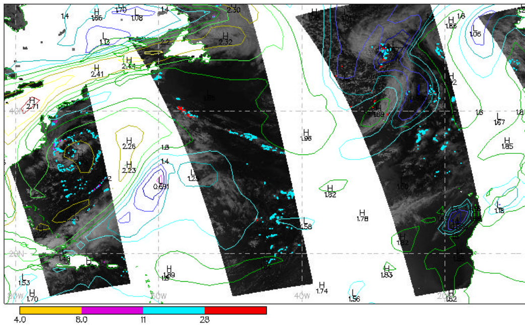
Figure 1. Sulfate column amount (contours) in \log_{10}(\mu\text{moles}/\text{m}^2) simulated by the chemistry model over the North Atlantic for 1800 UTC on April 21, 1987. Superimposed are channel 1 (Visible) images from the AVHRR on NOAA-10 for three overpasses spanning the same time period. Retrieved cloud drop effective radius ( \mu\text{m} ) for clouds screened for temperature are shown in color.
